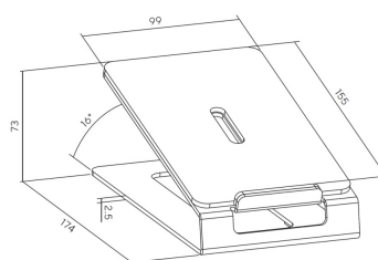
Dimensions (mm)
